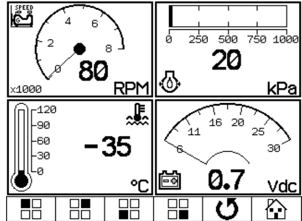
Customize Common Display Gauge Screen
