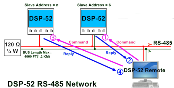
DSP-52 Remote RS-485 Network
