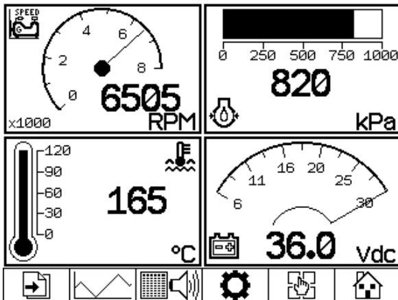
Graphical Gauge Menu bar screen
