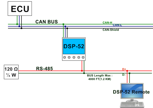
DSP-52 Network Structure Diagram
